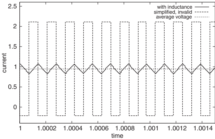
FIGURE 5.13 Comparison of the current for a 50% duty cycle in the original model, invalid simplified model, and average voltage.
