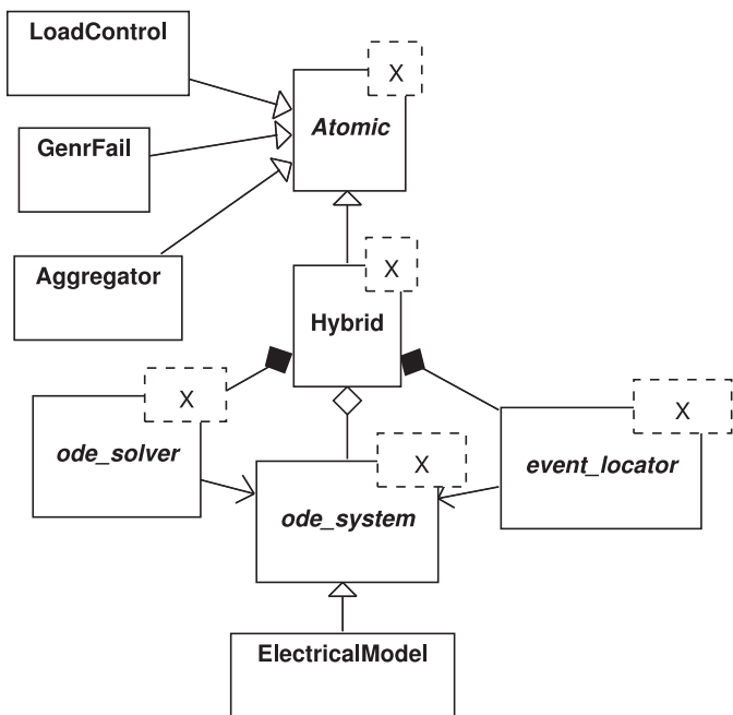
FIGURE 6.14 Class diagram of the model's power and control elements.
