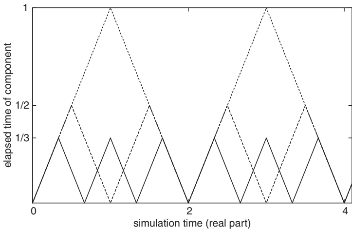
FIGURE 5.19 The clock variables of a differential automaton with component periods of 1, \frac{1}{2} , and \frac{1}{3} ; its “smaller” asynchronous automaton is shown in Figure 4.13.
