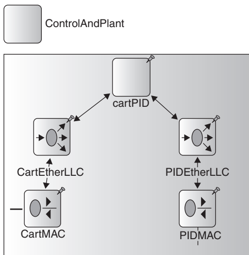
FIGURE 6.4 Diagram of the CartPID protocol stack (below) and the Ethernet network (above).
