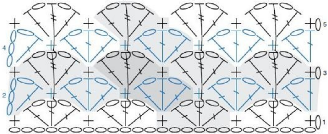
Corded Shells Cowl Top Reduced Sample of Stitch Diagram Note: Reps shown in gray.
