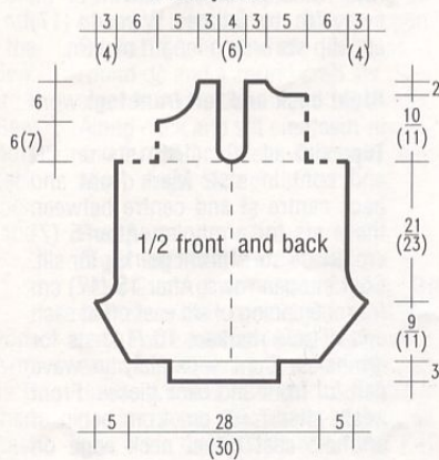
1/2 front and back
