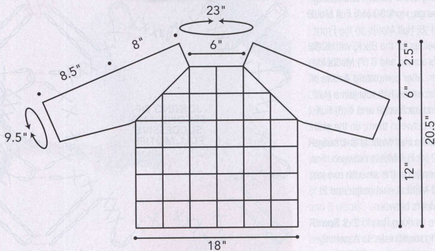
ASSEMBLY DIAGRAM SIZE S/M
